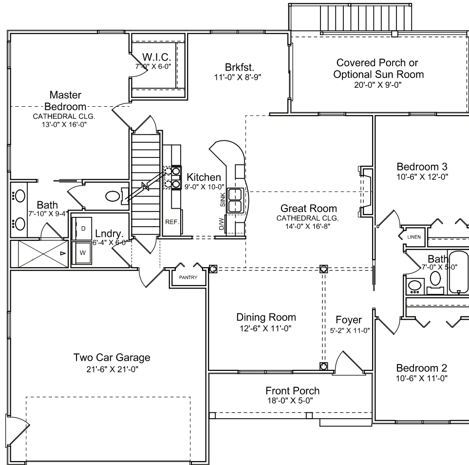
FLOOR PLAN 1,556 SQUARE FEET
