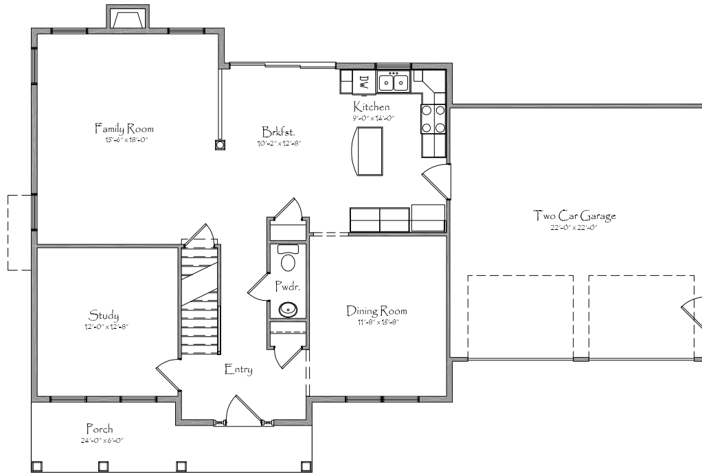
FIRST FLOOR PLAN 1,117 SQUARE FEET
