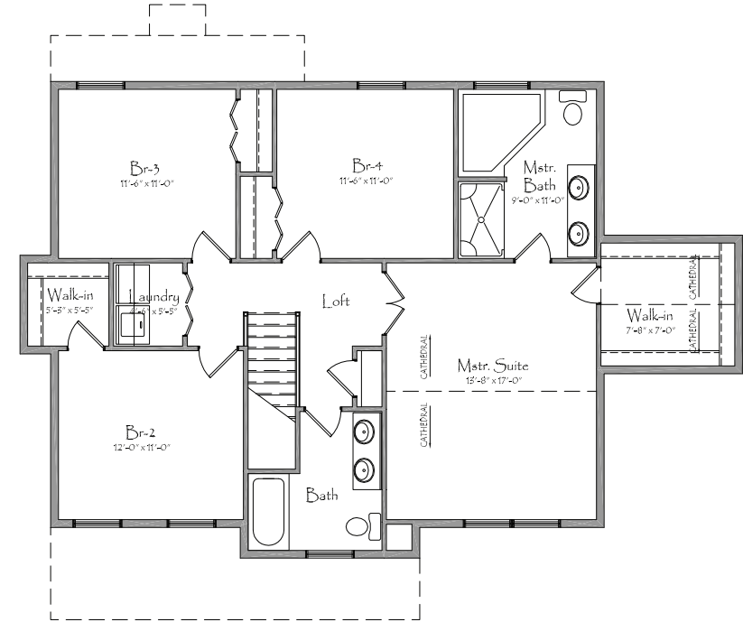
SECOND FLOOR PLAN 1,162 SQUARE FEET
