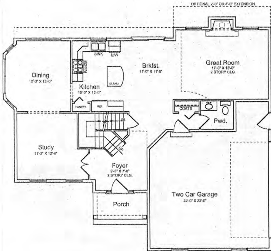
FIRST FLOOR PLAN 1,112 SQUARE FEET
