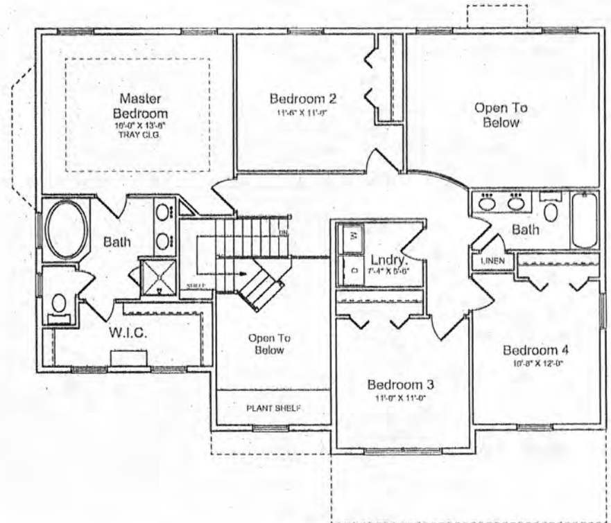
SECOND FLOOR PLAN 1,165 SQUARE FEET
