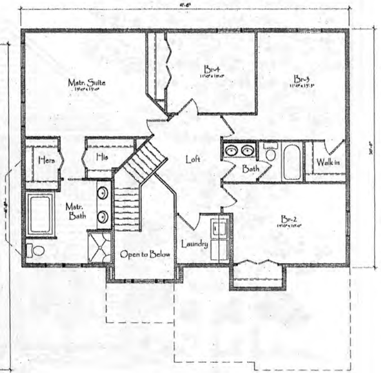
SECOND FLOOR PLAN 1175 SQUARE FEET
