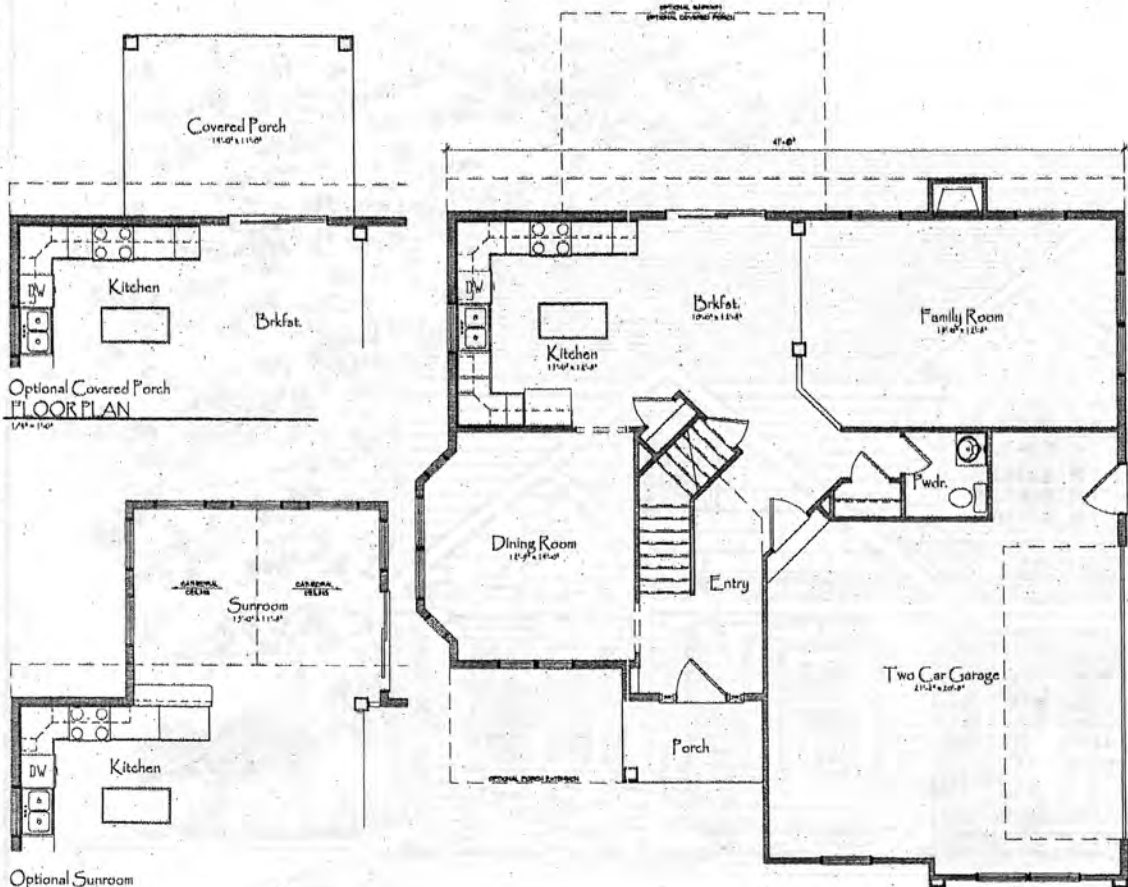
FIRST FLOOR PLAN 947 SQUARE FEET
