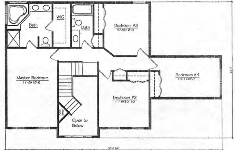
OPT. SECOND FLOOR PLAN 1,110 SQUARE FEET
