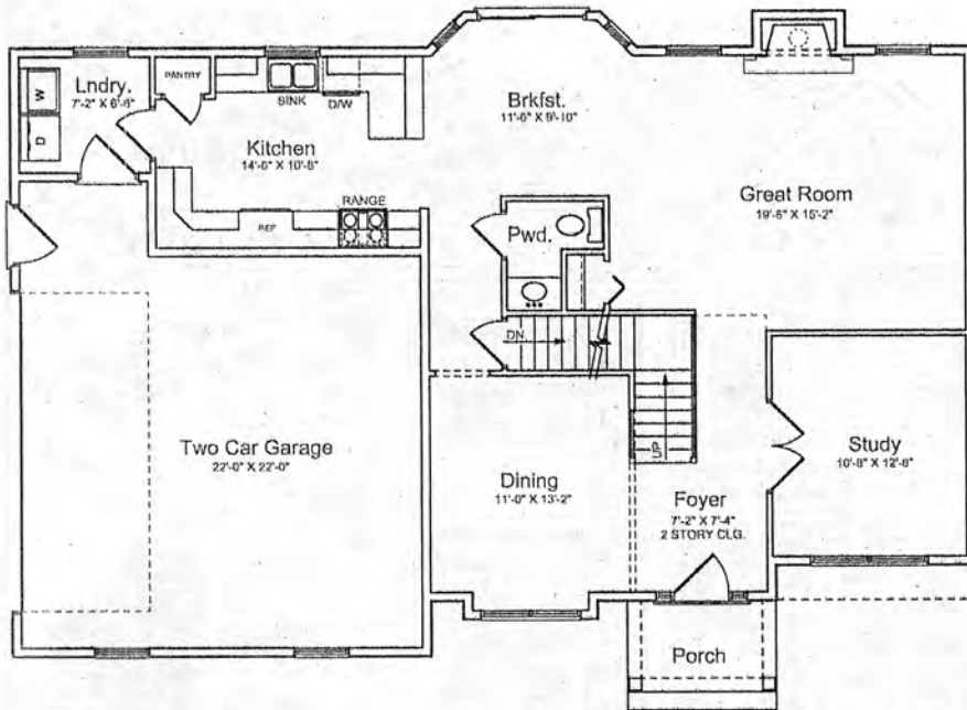
FIRST FLOOR PLAN 1,167 SQUARE FEET
