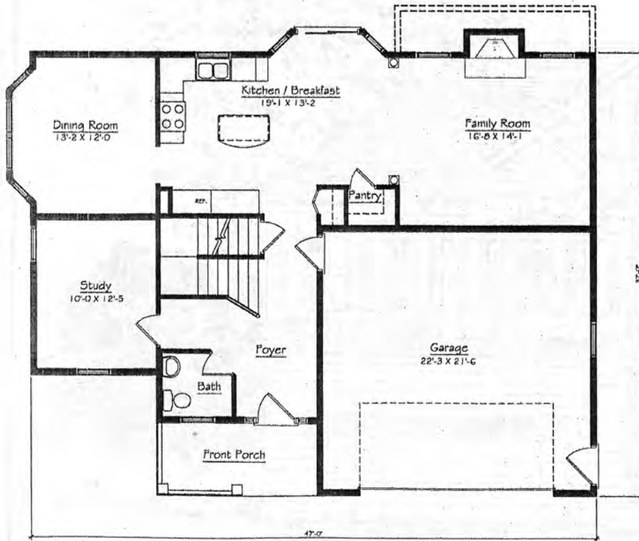
FIRST FLOOR PLAN 1,087 SQUARE FEET
